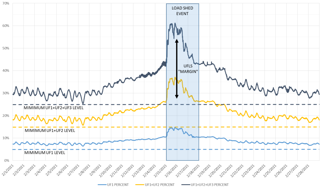
Figure 1: February cold event UFLS connected load percentages (Feb 15-16 in blue shade area)
